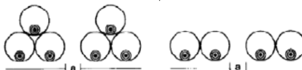
Cables unipolares
